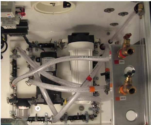
Raw water pump and filter assembly
