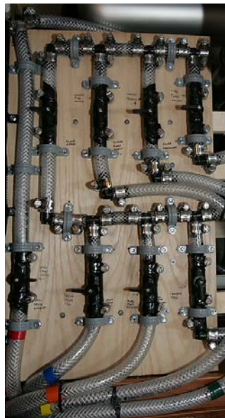
Fresh water valve array
