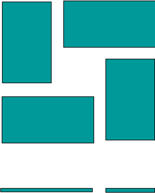
Solar Cells
